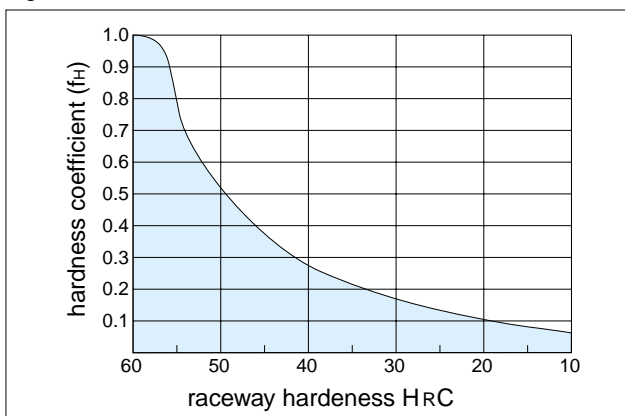
Figure C-4: Hardness coefficient
